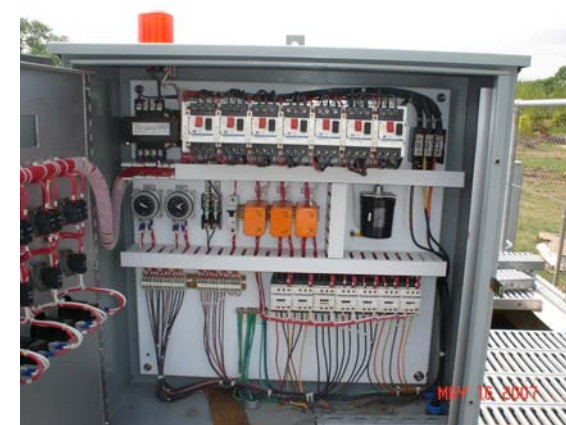
Fig. 6) Control Panel for WWTP and Dosing Tank
